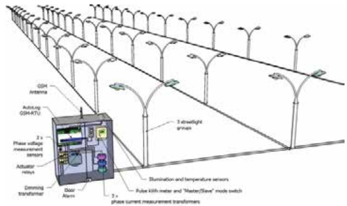
Smart Street Lighting System
