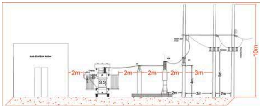
10/12.5MVA, 33/11KV, Outdoor Substation
